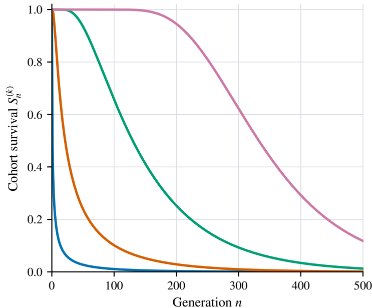
Subcritical: p = 0.495
