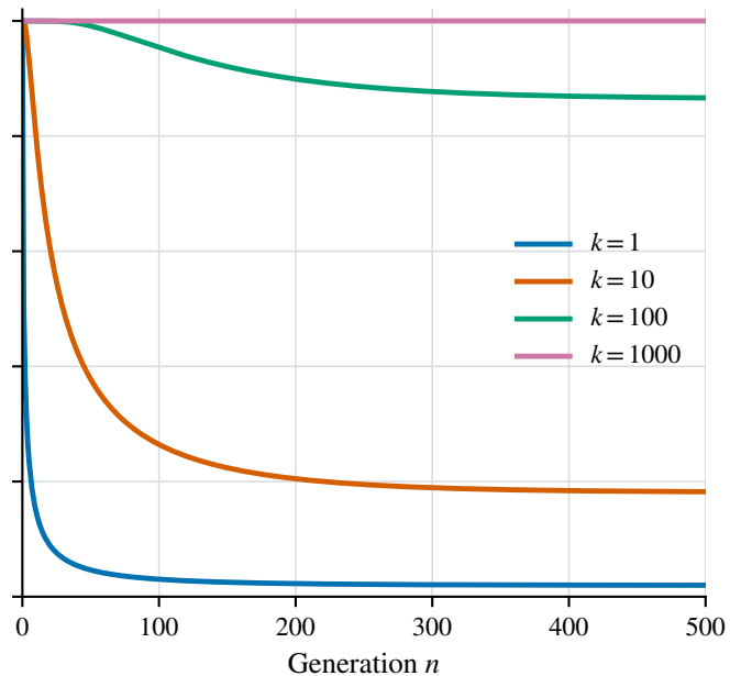
Supercritical: p = 0.505
